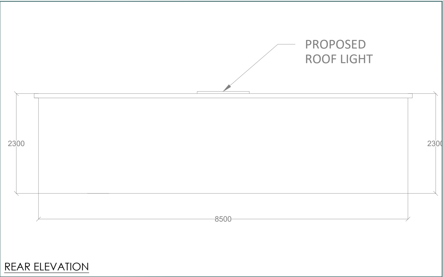
REAR ELEVATION
